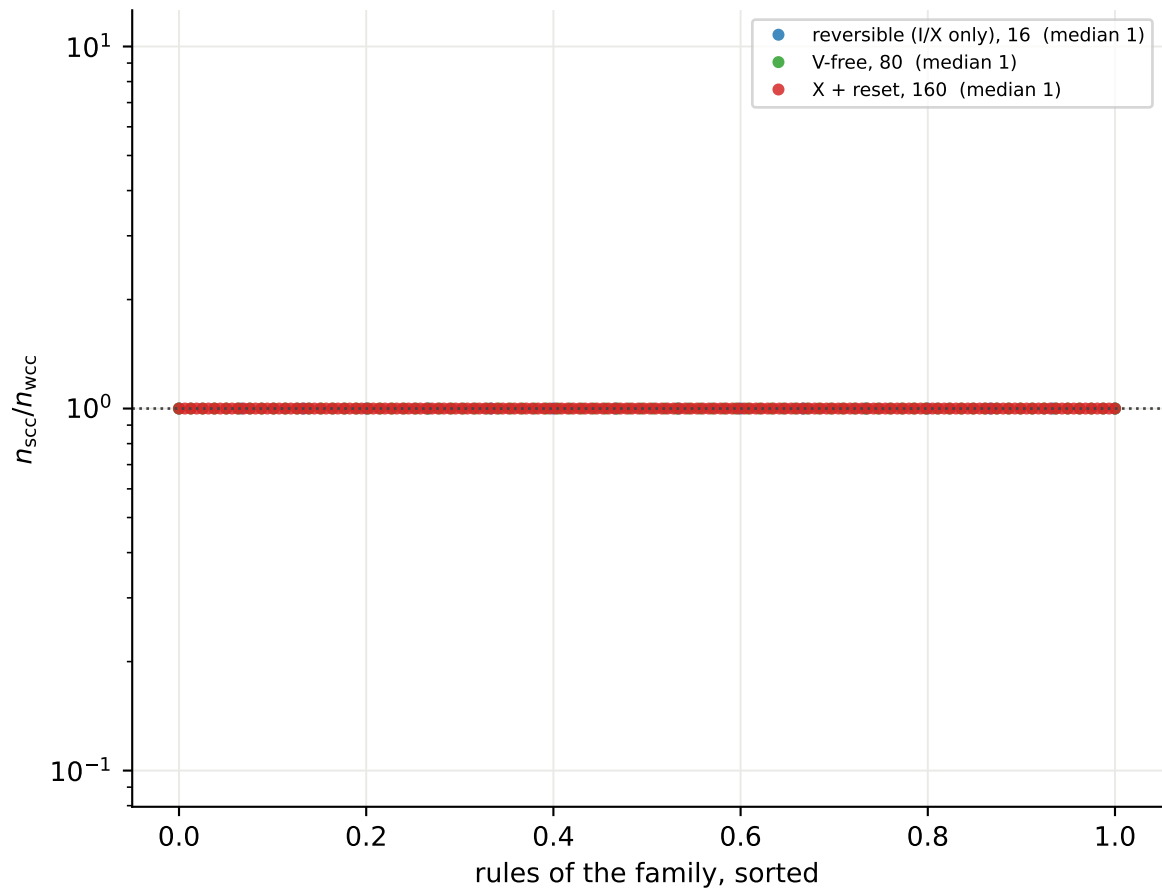
X8b the same as a per-rule ratio, each family sorted: how many attractors a sector carries
