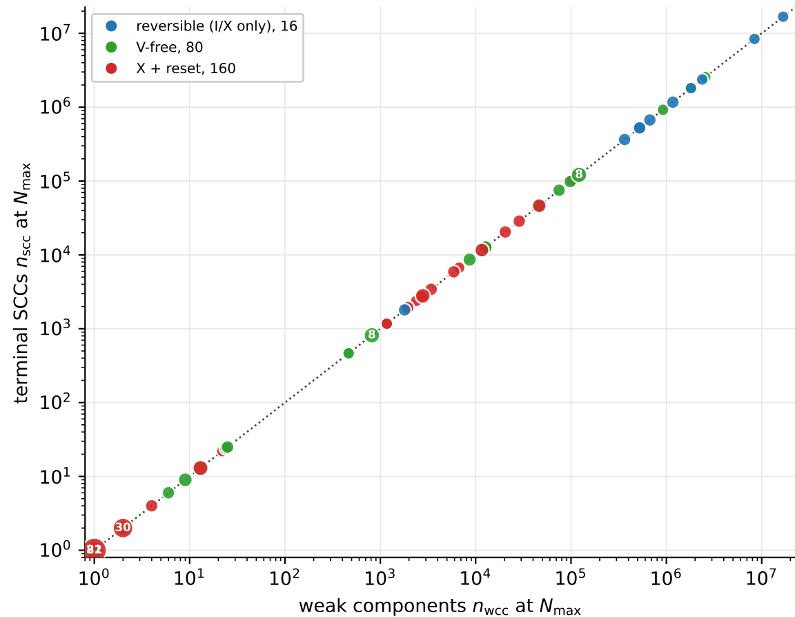
X8a X gate: weak components against terminal SCCs (raw counts) 256 of 256 rules sit exactly on the diagonal
