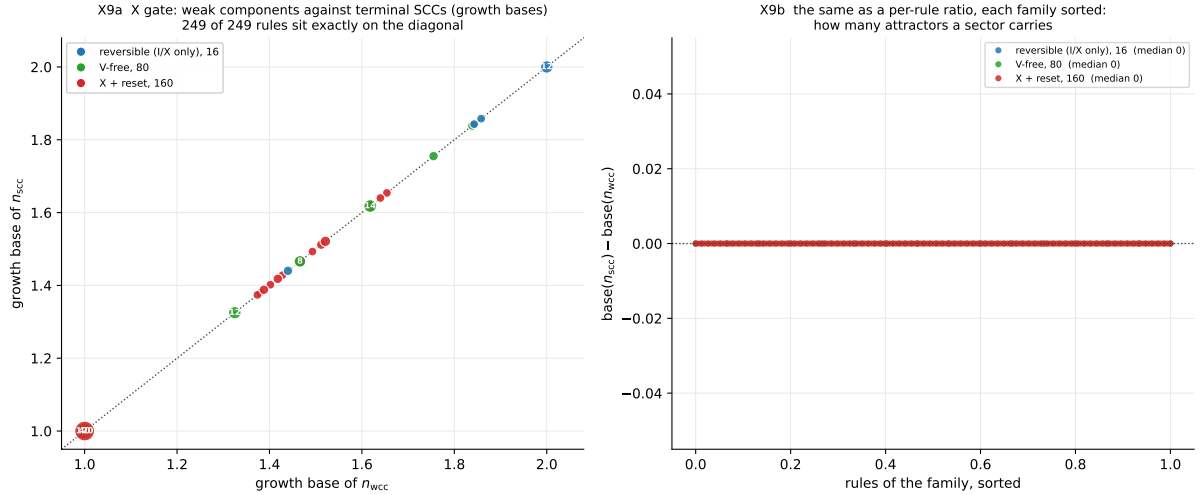
Figure 9: X9, the same in growth bases (obc0) . All 249 rules with both descriptors sit on the diagonal.
