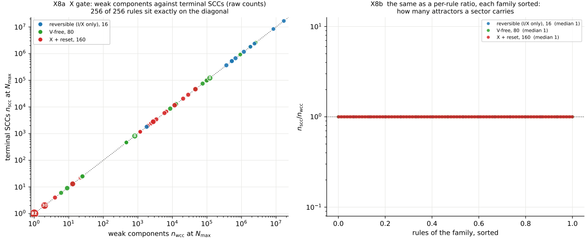
Figure 8: X8, weak components against cycles: raw counts (obc0) . Every one of the 256 rules sits on the diagonal at every N . Compare R9's F11, where twelve rules do not.
