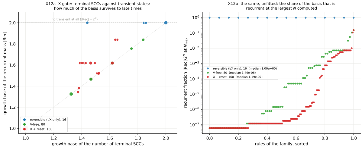
Figure 12: X12, cycles against transient states (obc0) . Left: growth base of the number of cycles against that of the recurrent mass |Rec| . Right: the recurrent fraction at the largest N , each family sorted.
