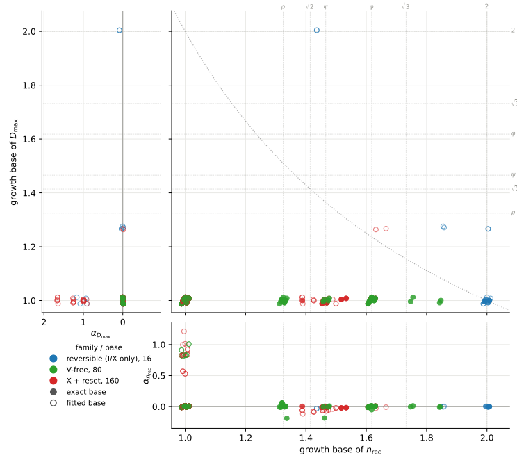
Figure 11: X11, the same for the cycles (obc0) . By the identity above the horizontal axis is the same axis as X10's; only the vertical one changes, from the largest sector to the longest cycle.
