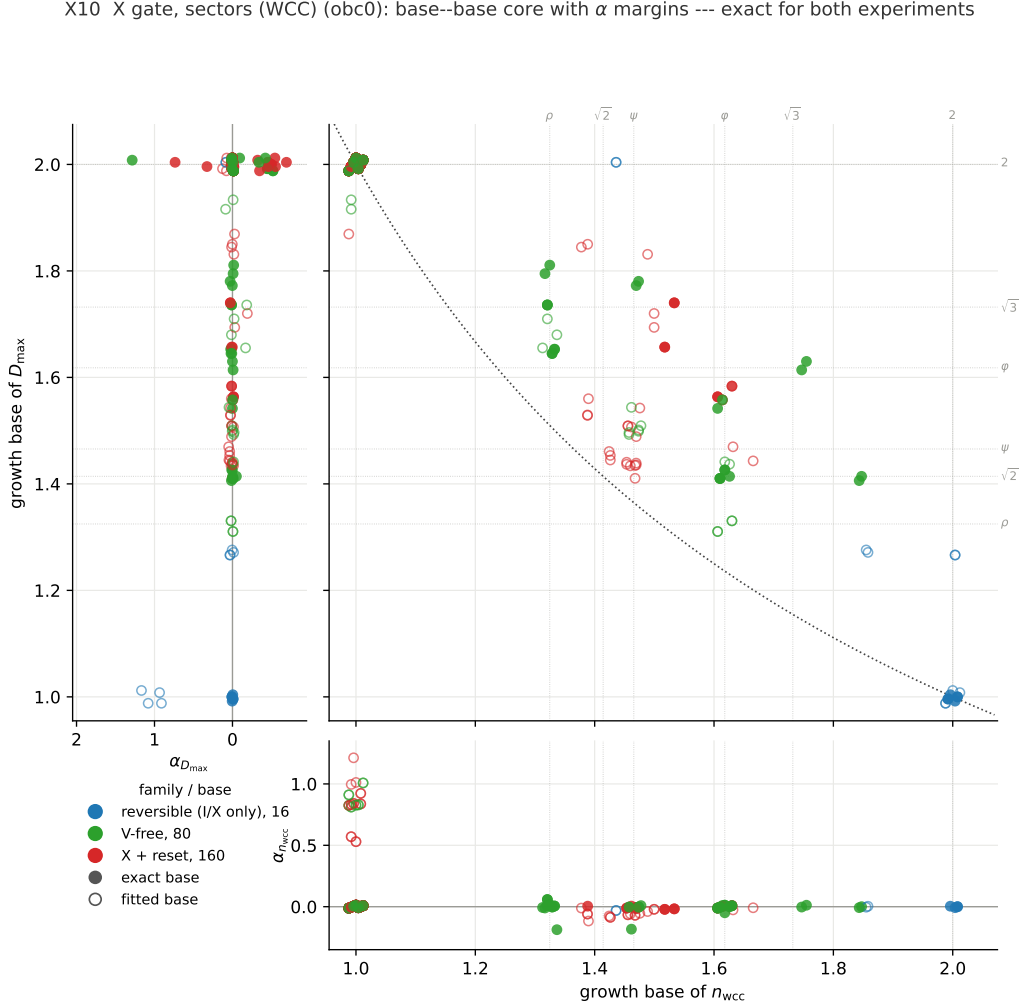
Figure 10: X10, the X-gate sector map in corner form (obc0) . Main panel: base--base. Bottom margin: the sector count's sub-leading power; left margin: the D_{\max} power. Filled marker = exact base.
