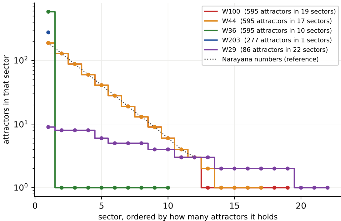
How the attractors distribute across sectors ( N = 16 )
