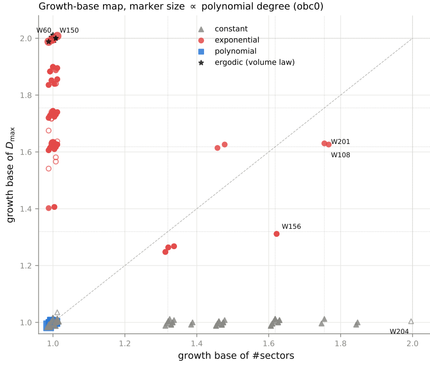
Figure 5: Companion base-vs-base map (obc0): growth base of the sector count against that of D_{\max} , marker size \propto polynomial degree, ergodic rules as stars. The corners read directly: bottom-right = shattered into O(2^N) frozen sectors (204), top-left = a single volume-law sector (ergodic and the domain-wall family), diagonal = both count and size grow exponentially.
