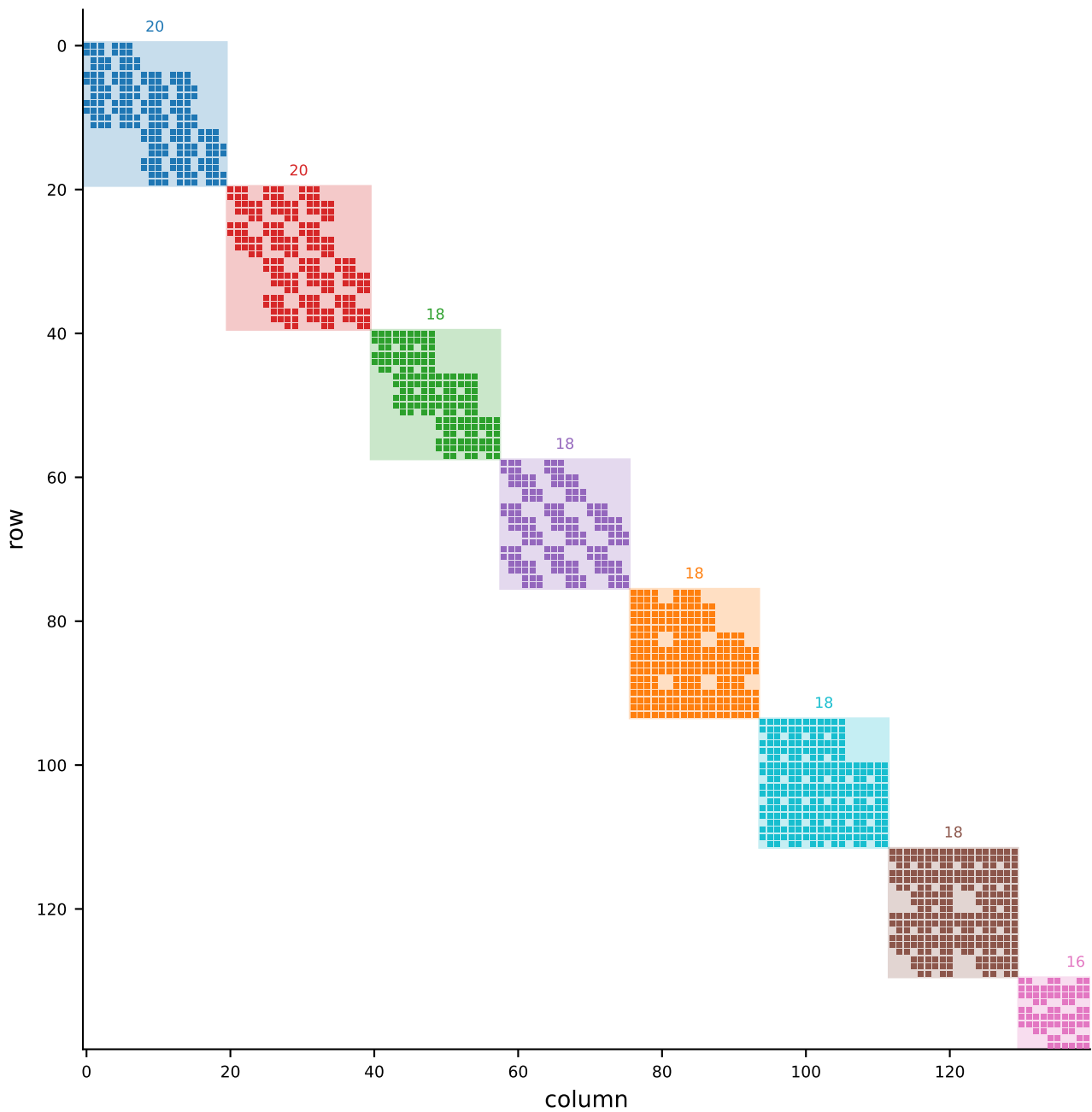
W156 obc0 N = 10 : first 140 rows/columns of the sorted matrix (block sizes annotated)
