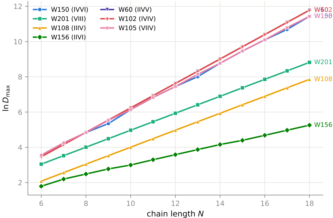
Largest sector vs system size (obc0)
