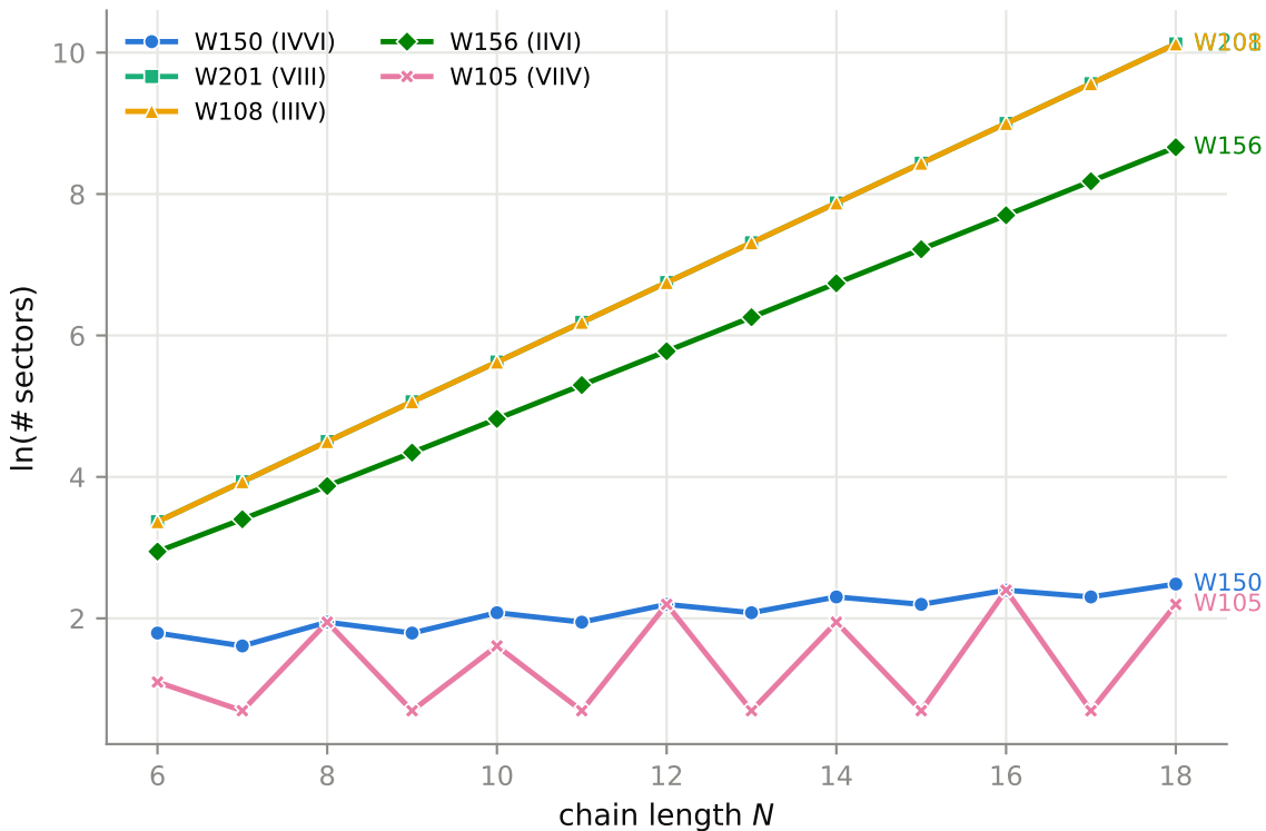
Sector count vs system size (pbc)
