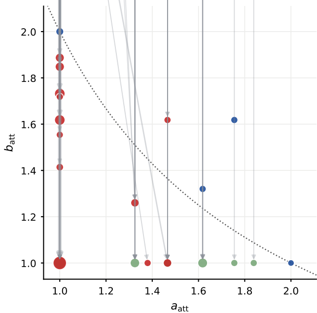
attractors (terminal SCC)
