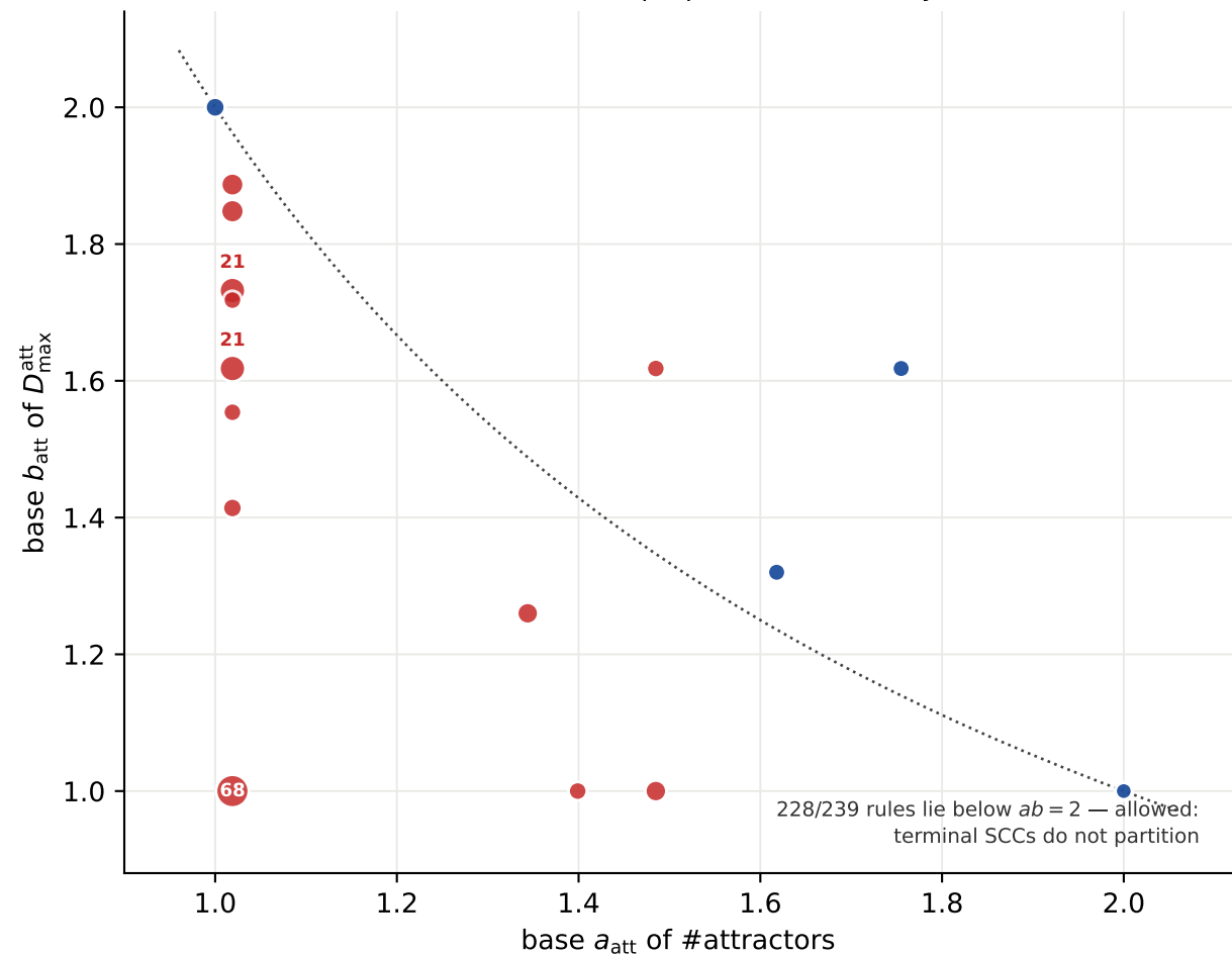
monitored attractor map, quantum rules only (obc0)
