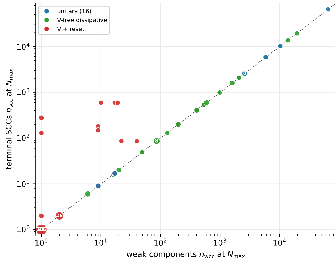
F11a Hadamard gate: weak components against terminal SCCs (raw counts) 237 of 249 rules sit exactly on the diagonal
