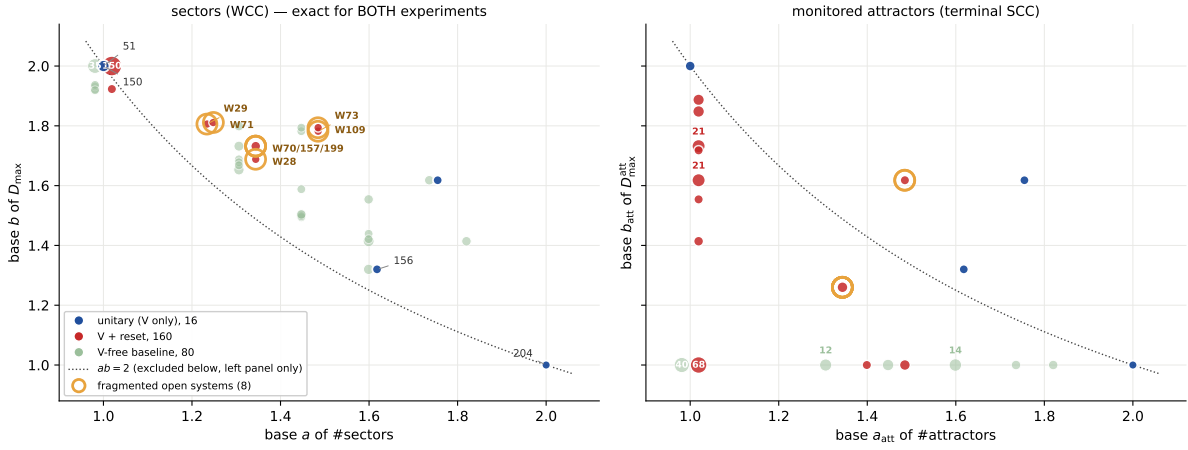
Figure 1: F1, the two maps on identical axes. Left: the sector (WCC) plane, base a of the sector count against base b of the largest sector — exact for both experiments . Right: the same plane for terminal SCCs — monitored only . The dotted line is ab = 2 ; it excludes the region below it in the left panel and is only a reference in the right one. Marker area grows with the number of rules stacked in a cell and the count is printed inside crowded cells, without which the distribution is invisible: 77% of the sector map lies in one cell. Colour is by family, with the quantum rules (those carrying a Hadamard) drawn forward and the V-free rules held back as a baseline. Gold rings and labels mark the eight V+reset rules that stay exponentially fragmented (§9.2). The nine unitary rules land at identical coordinates in both panels, which is assertion A2 made visible. The three families are drawn with a horizontal offset of \pm 0.019 (V+reset right, V-free left, unitary unshifted): without it the 144 V+reset rules at (1,2) sit exactly under 33 V-free ones and one family is invisible. Positions within a family are therefore exact relative to each other, but an absolute base read off the axis carries that offset — take exact values from the tables, not from the figure.
