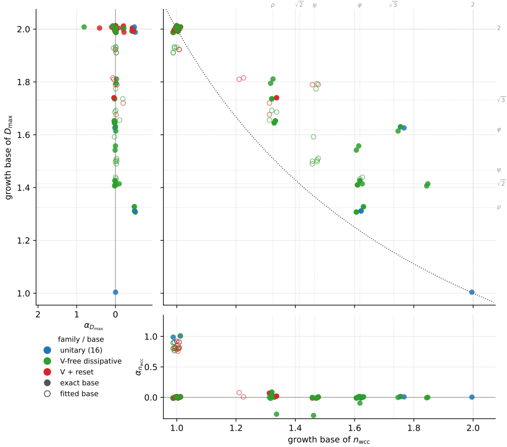
Figure 4: F8, the sector map in corner form (obc0) . Main panel: the map of Figure 1 with the exclusion curve. Bottom margin: the sector count's sub-leading power against its base — the column at a = 1 splits into \alpha \simeq 0 (genuinely one sector) and \alpha \simeq 1 (the pinned-frontier rules of §9.5, a linear number of them), which the main panel cannot distinguish. Left margin: the D_{\max} power, where the binomial family's -\frac{1}{2} is visible at b = 2 . Filled marker = exact base.
