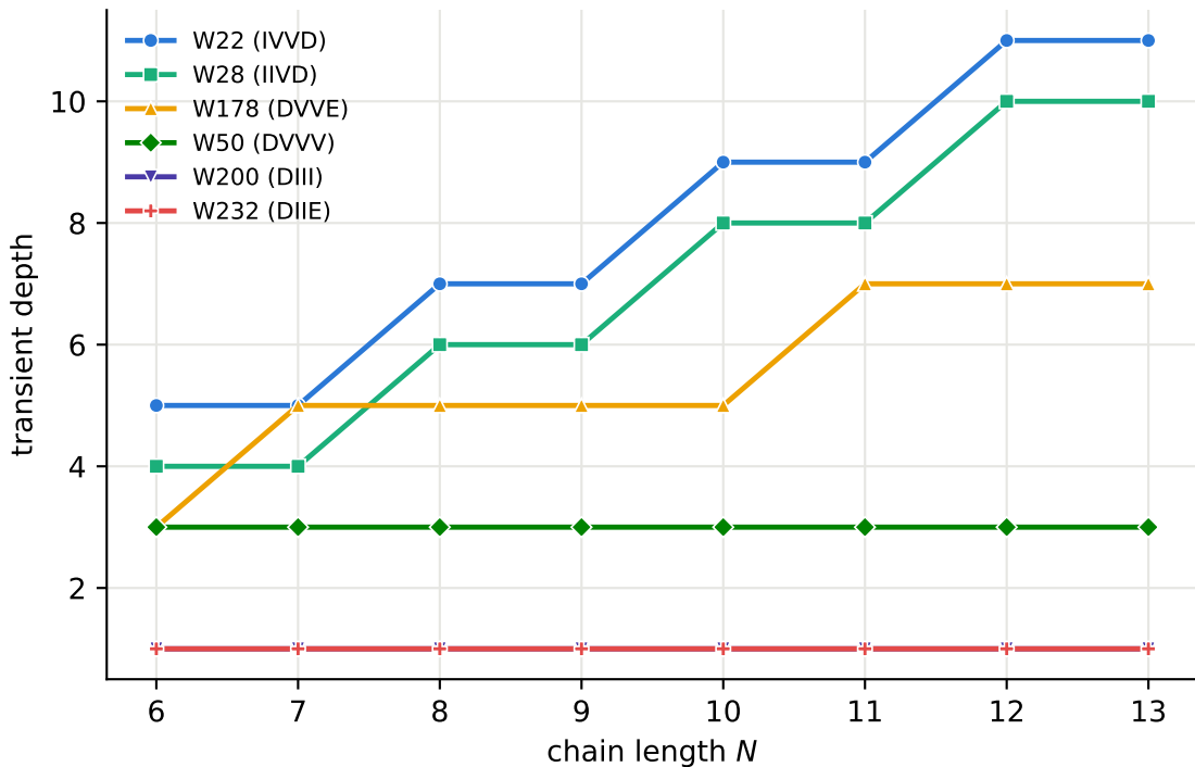
Relaxation (transient depth) vs N (pbc)
