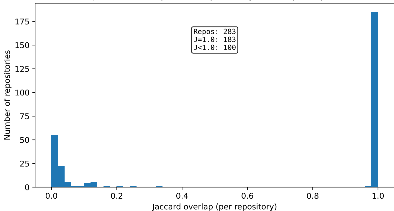
Jaccard overlap of attempted target sets (per repo)
