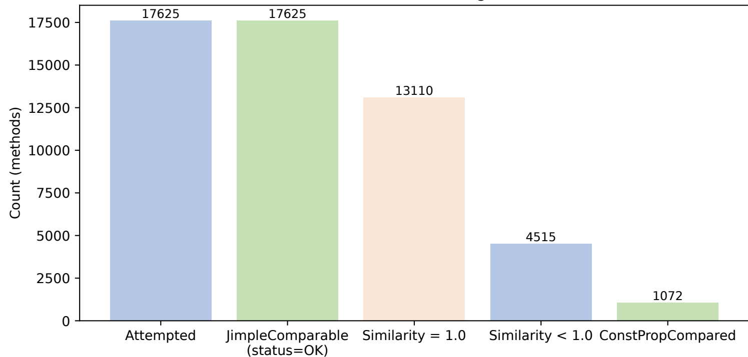
RQ3 Method funnel (coverage/attrition)
