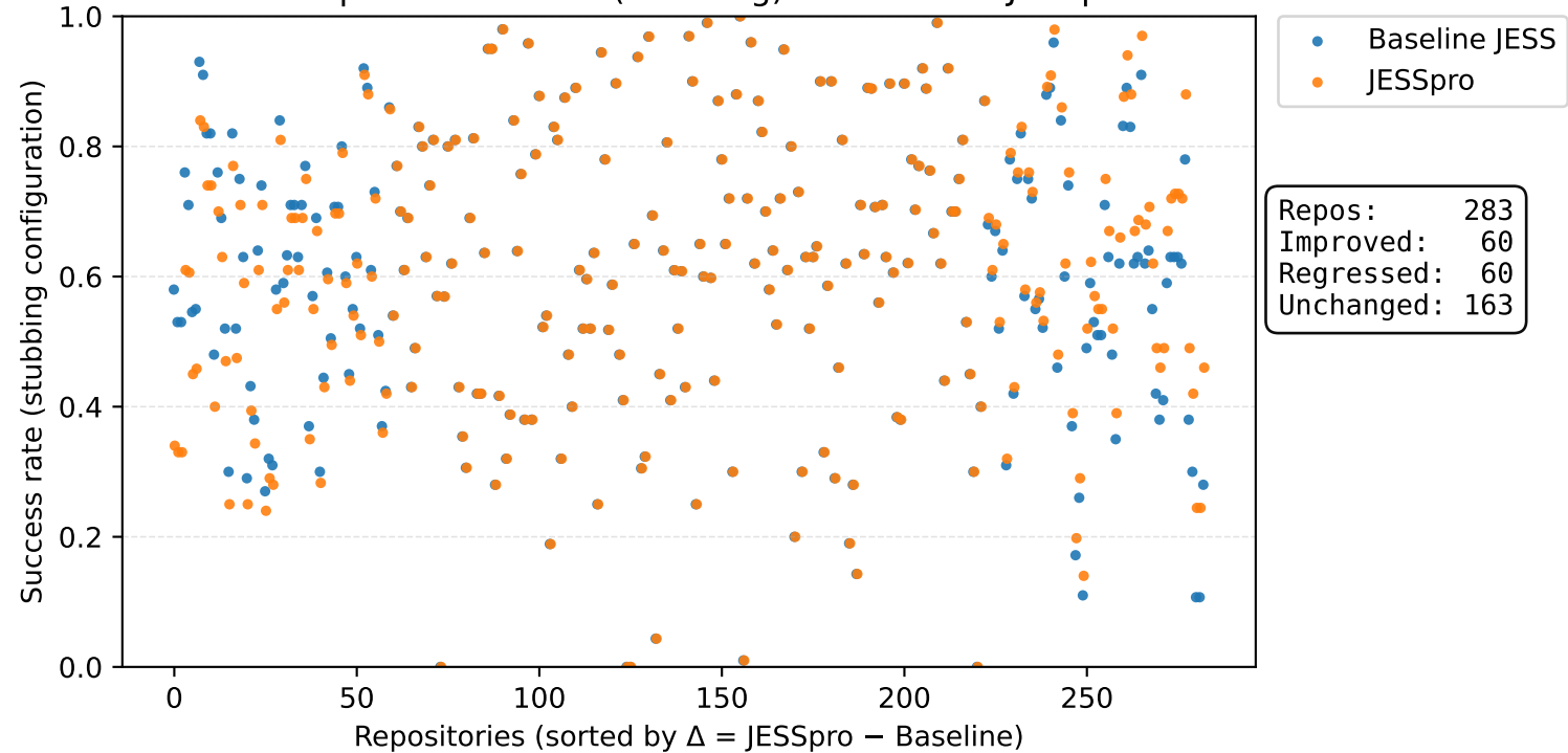
Per-repo success rate (stubbing): Baseline vs JESSpro
