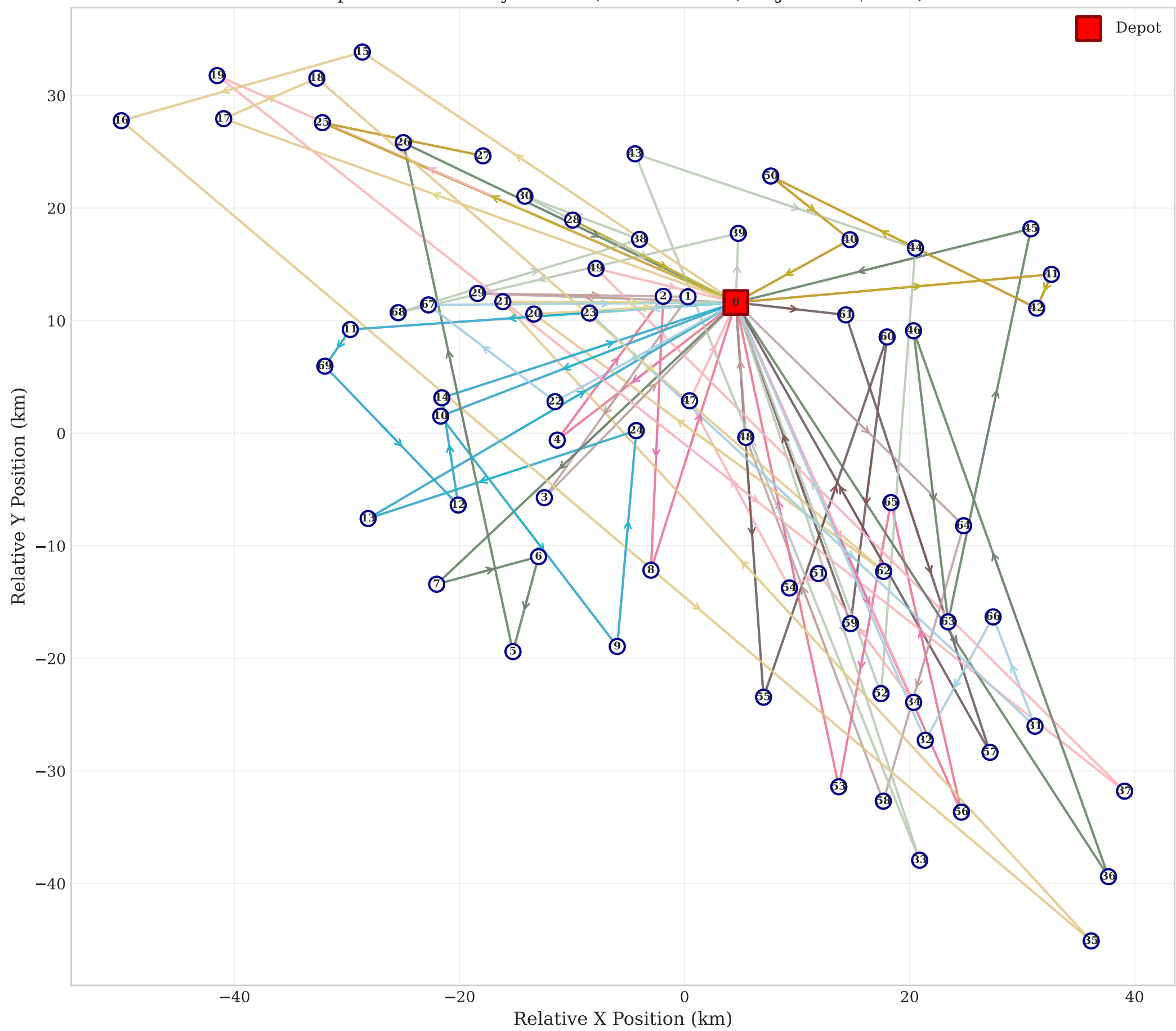
Optimized Delivery Routes (Fleet Size: 25, Objective: $5157)
