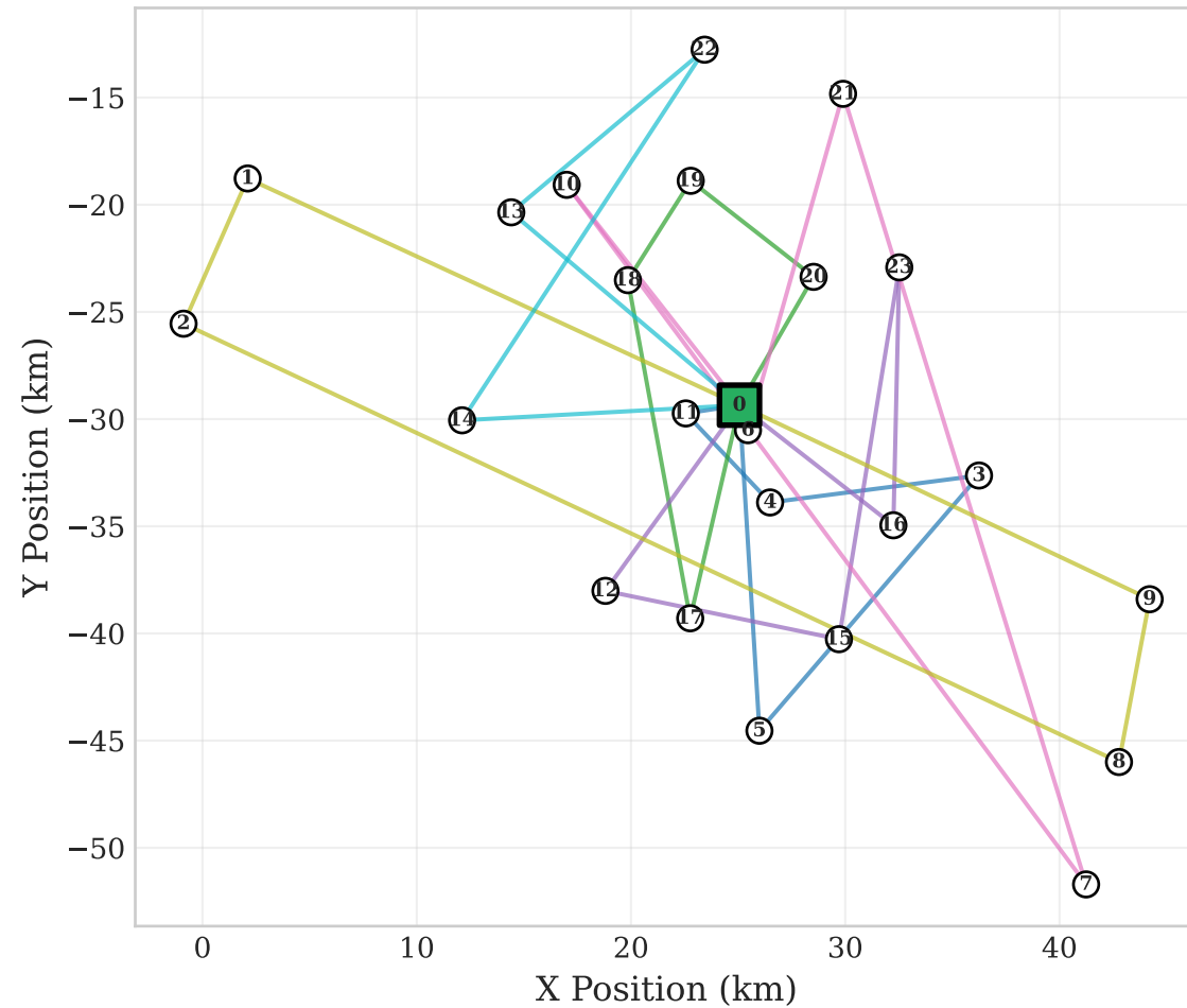
Depot 2 Routes (6 vehicles, $2173 cost)
