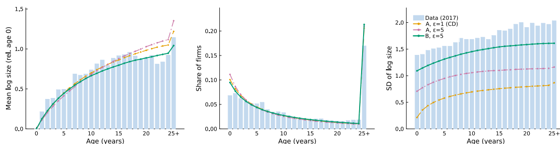
Figure 4: Fit of the three models: size, age distribution, and dispersion
