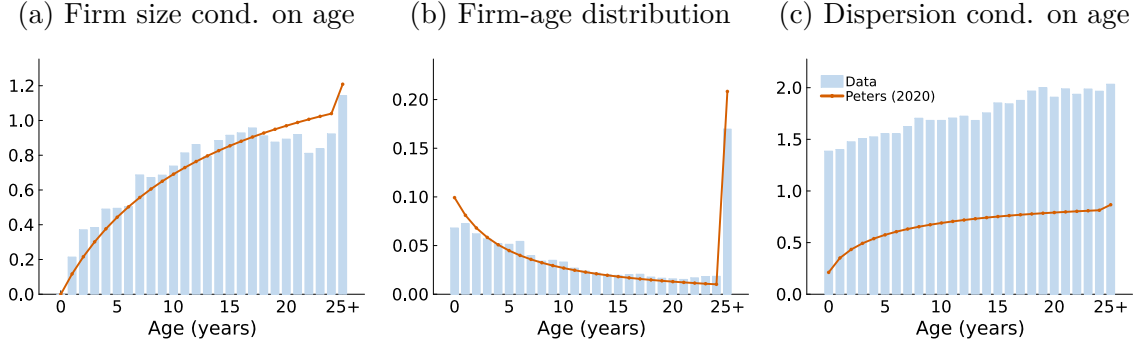
Figure A-4: Estimated Peters (2020) model: fit to the three margins
