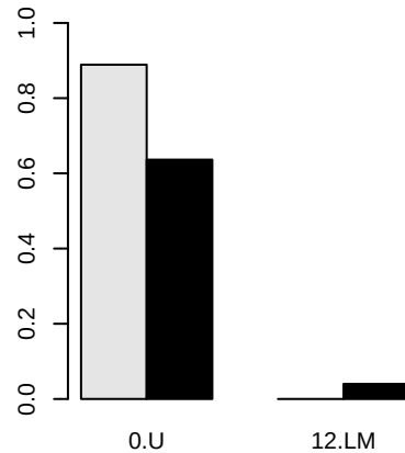
HETARB Green-Crown
