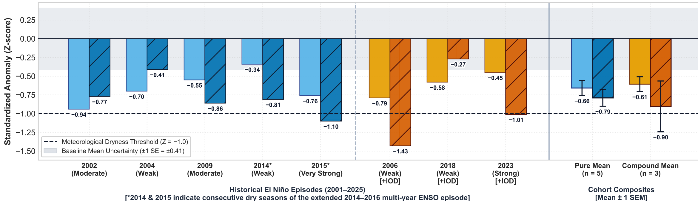
(b) Standardized Meteorological Anomaly (Z-score relative to ENSO-Neutral Baseline)
