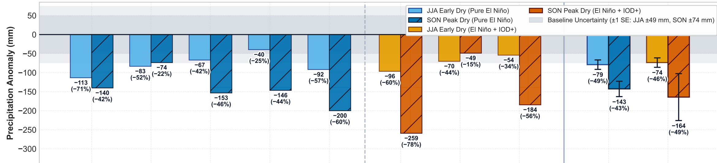
(a) Seasonal Precipitation Anomaly (mm) and Relative Departure (% of Climatological Baseline)
