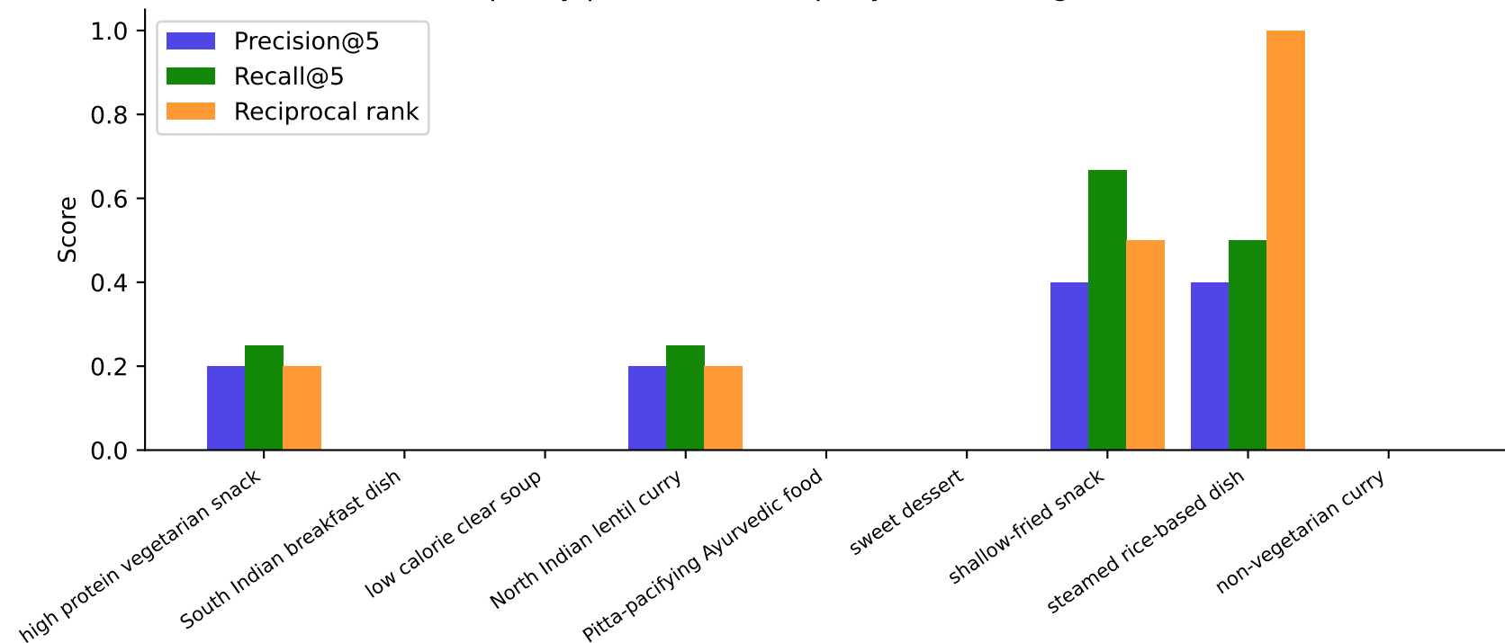
Retrieval quality per evaluation query (embedding: crc32-baseline)
