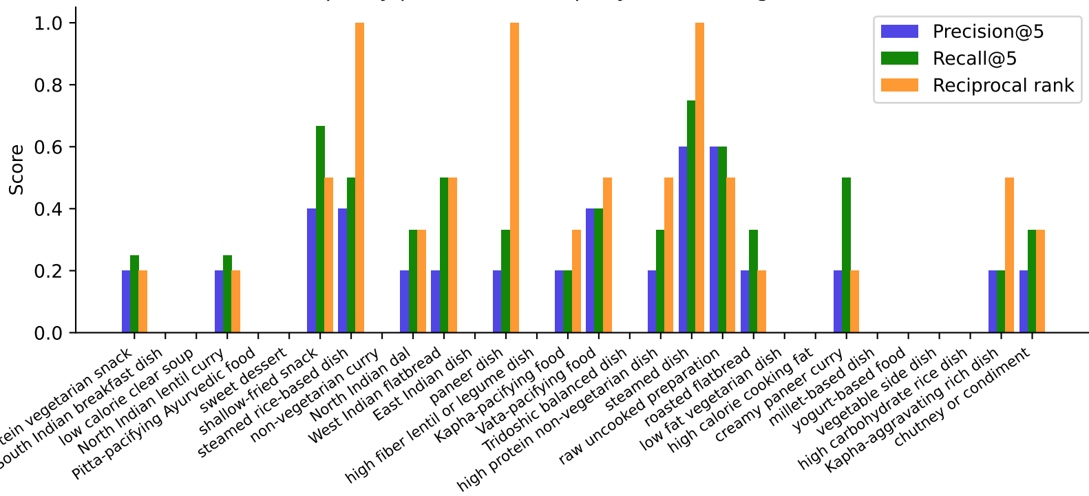
Retrieval quality per evaluation query (embedding: crc32-baseline)
