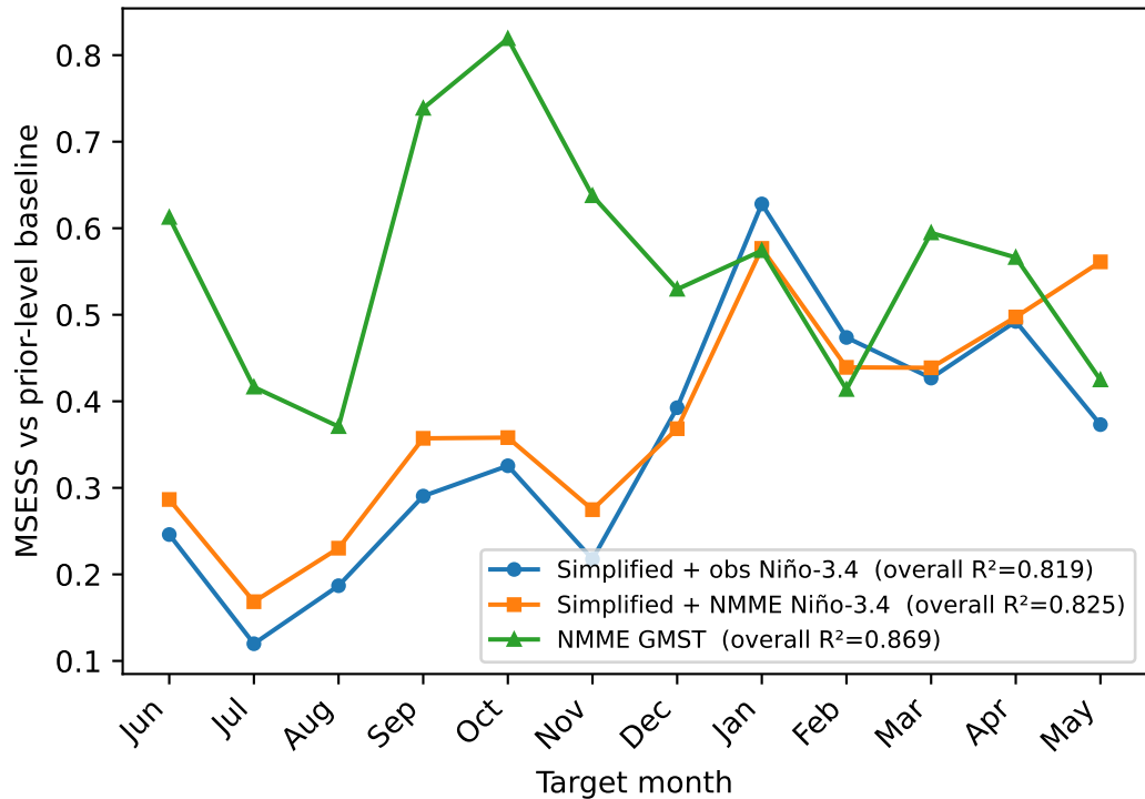
(b) MSESS vs prior-level baseline
