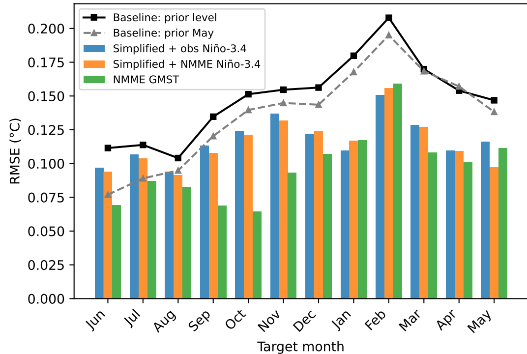
(a) RMSE by month (N=35, 1991-2025)
