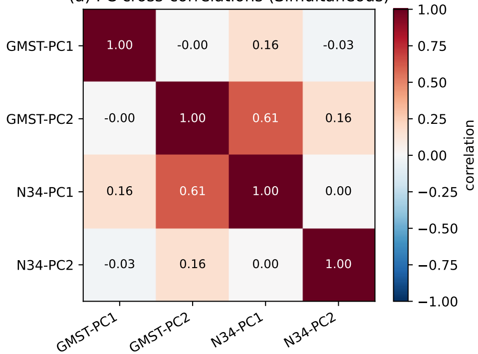
(a) PC cross-correlations (Simultaneous)
