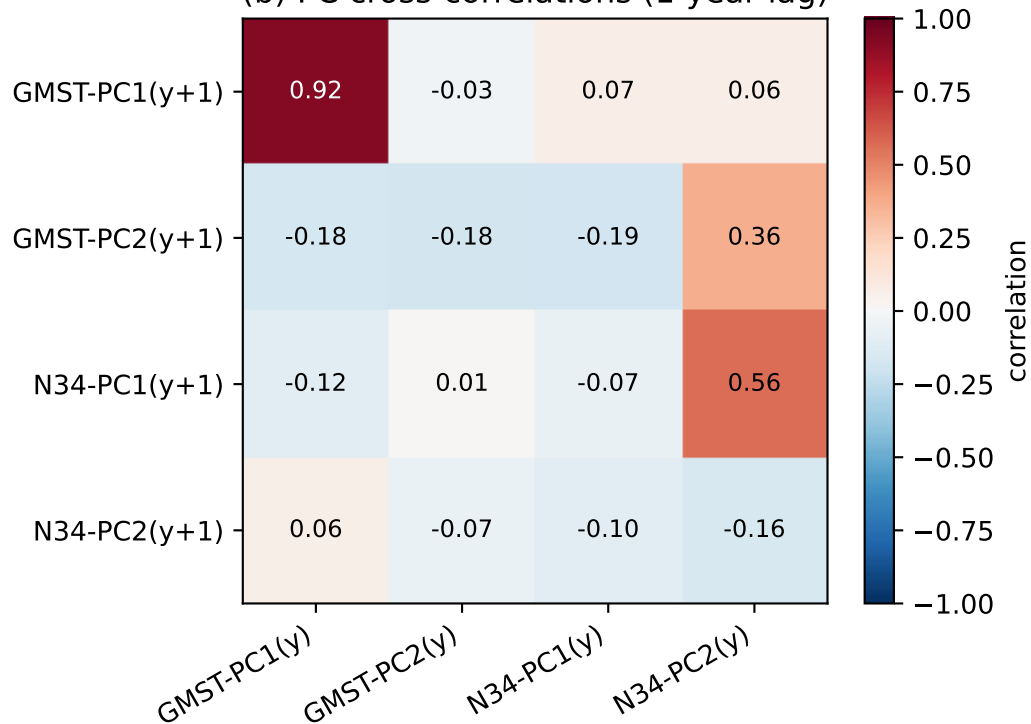
(b) PC cross-correlations (1-year lag)
