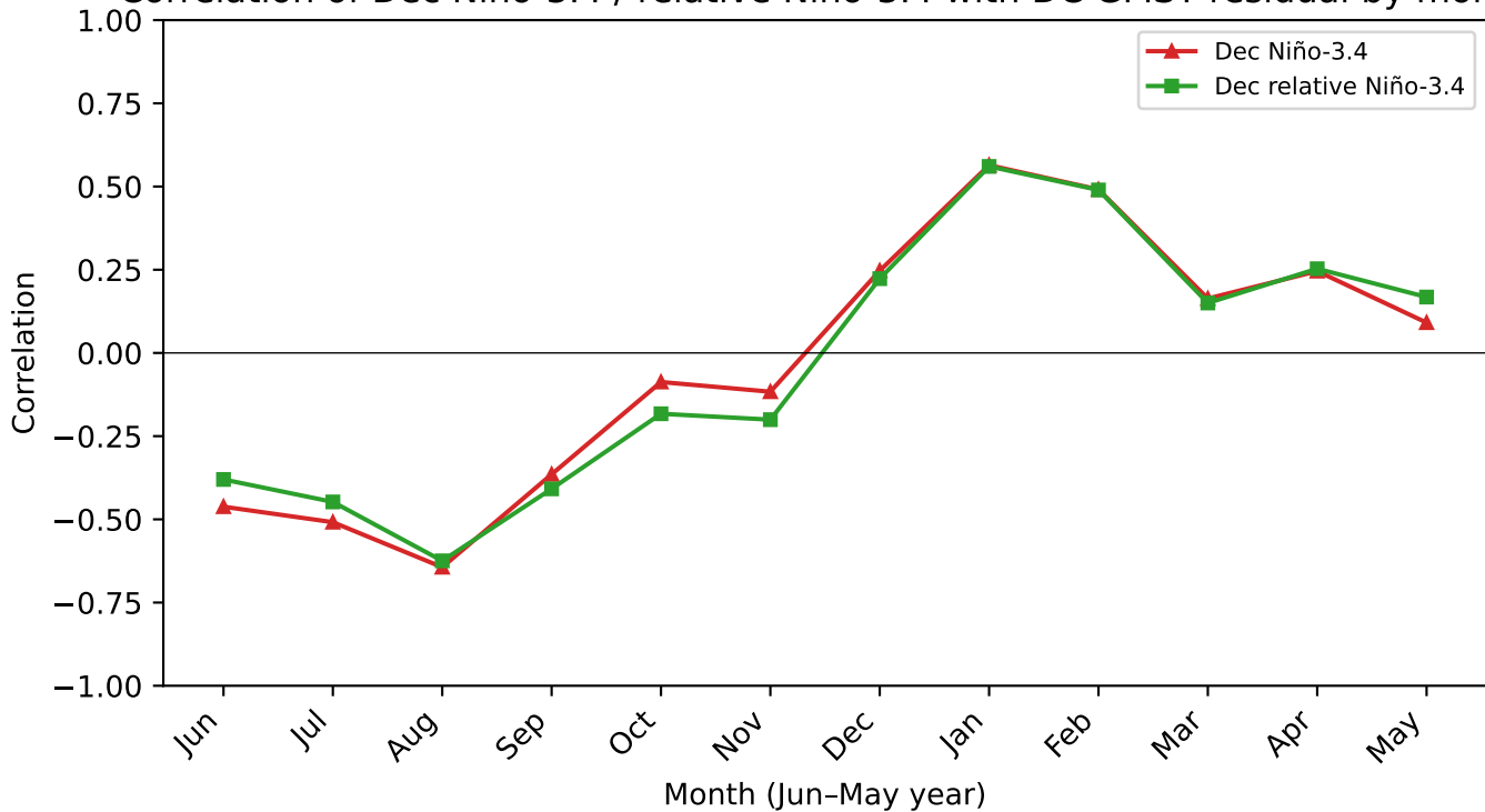
Correlation of Dec Niño-3.4 / relative Niño-3.4 with DC GMST residual by month
