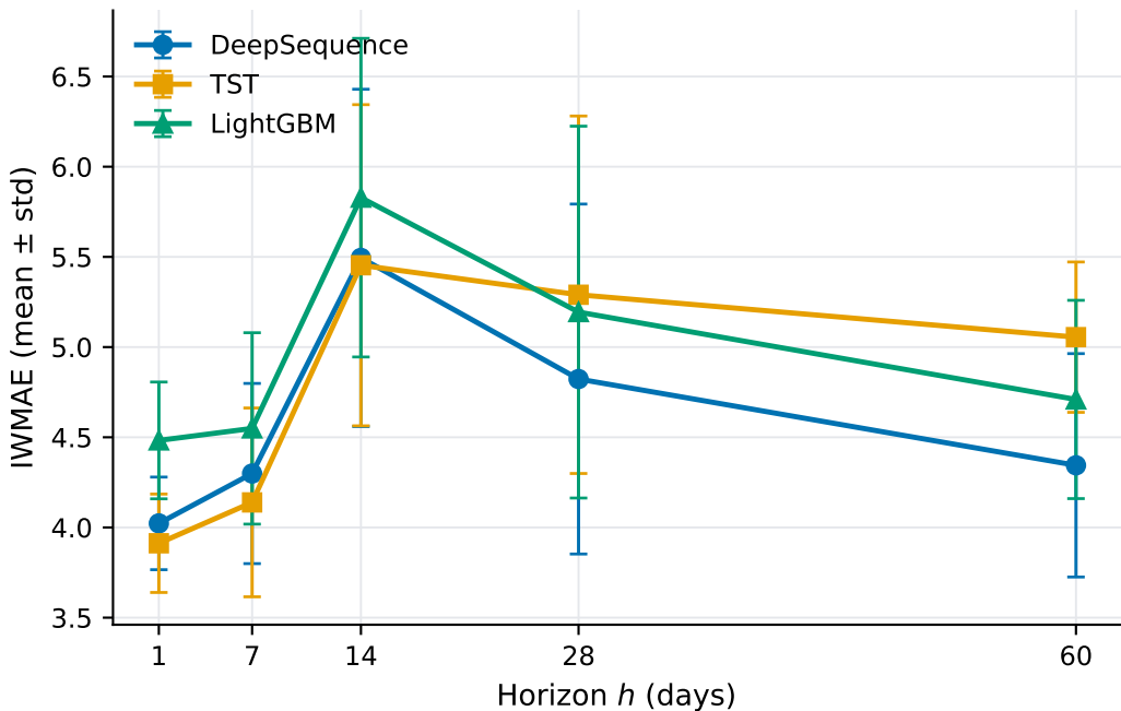
Daily multi-seed IWMAE vs horizon (seeds 42-46)
