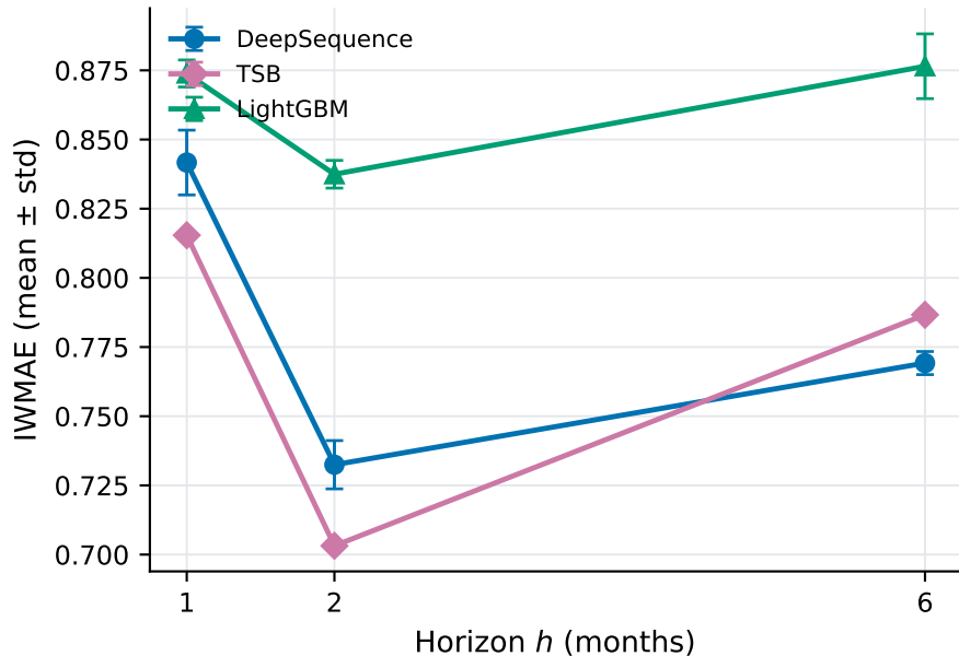
Car Parts multi-seed IWMAE
