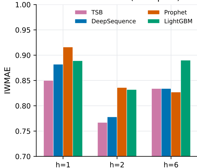
Seed-42 bake-off (+ Prophet)
