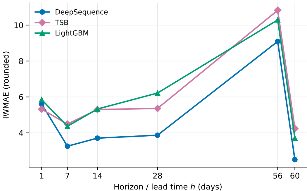
Daily Direct-MH IWMAE vs horizon (seed 42, locked 800)
