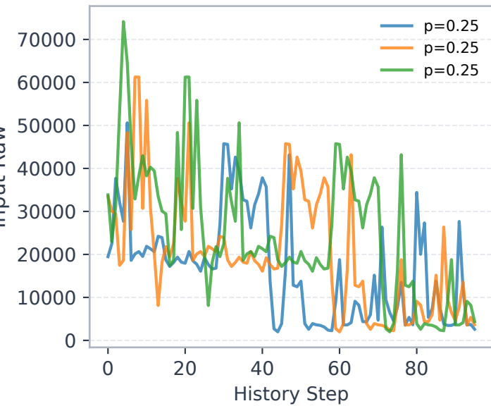
Geant E0
