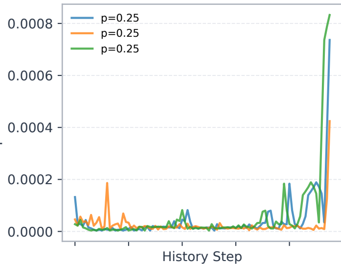
Geant E0
