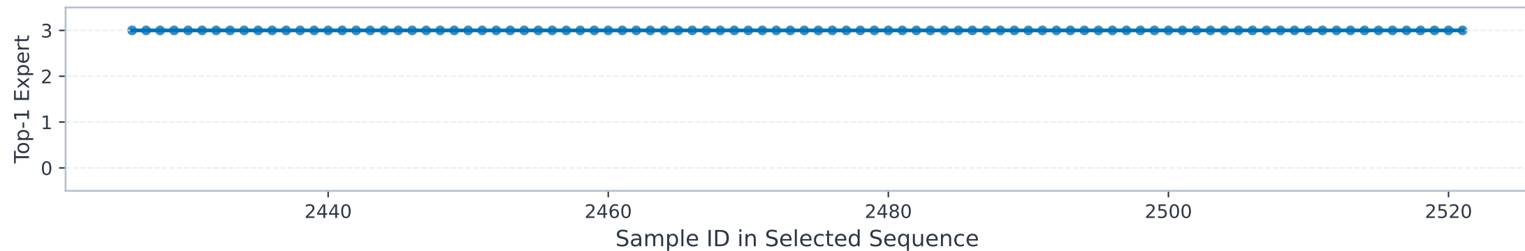
Geant
