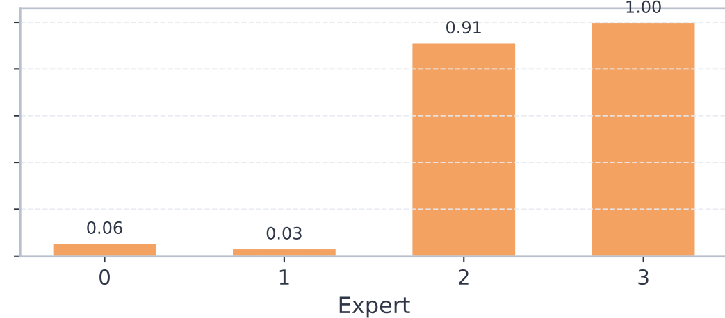
Geant
