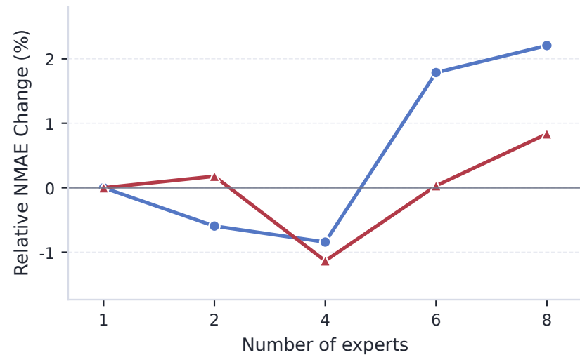
(a) Number of experts
