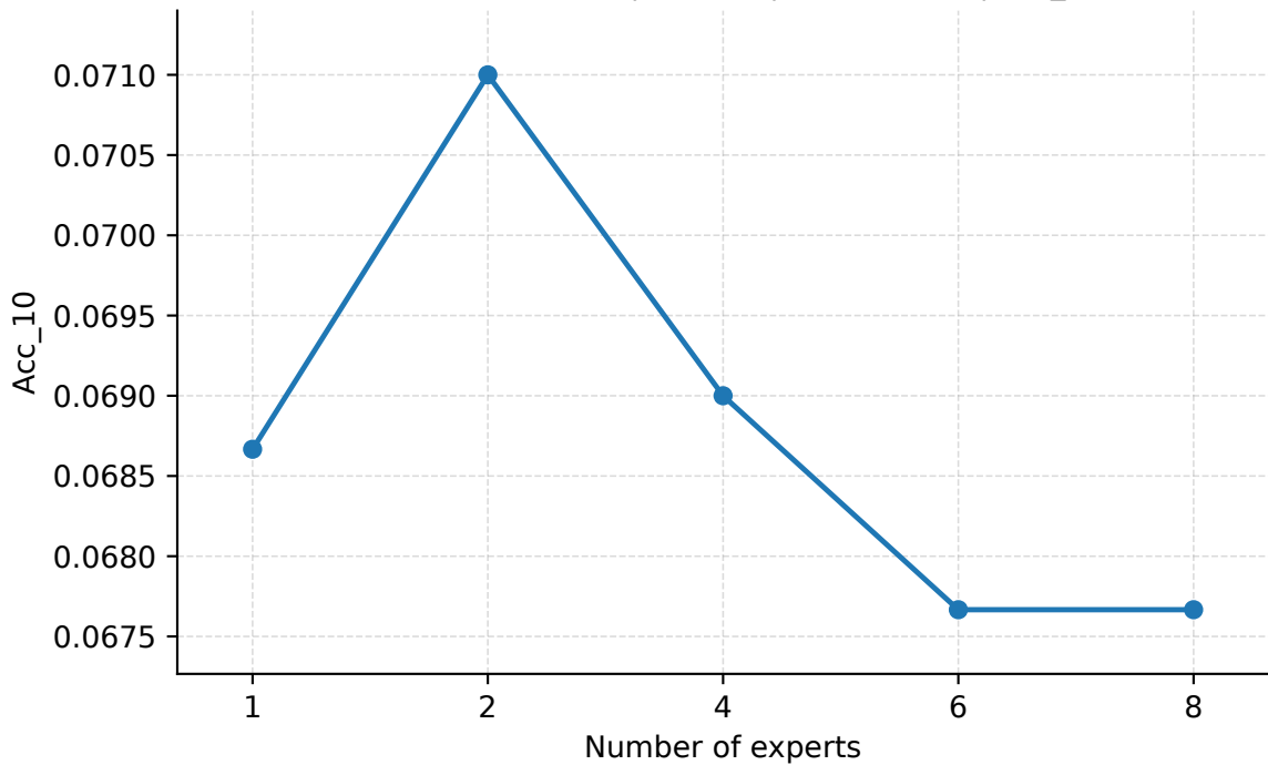
Number of Experts | Abilene | PredLen=10 | Acc_10
