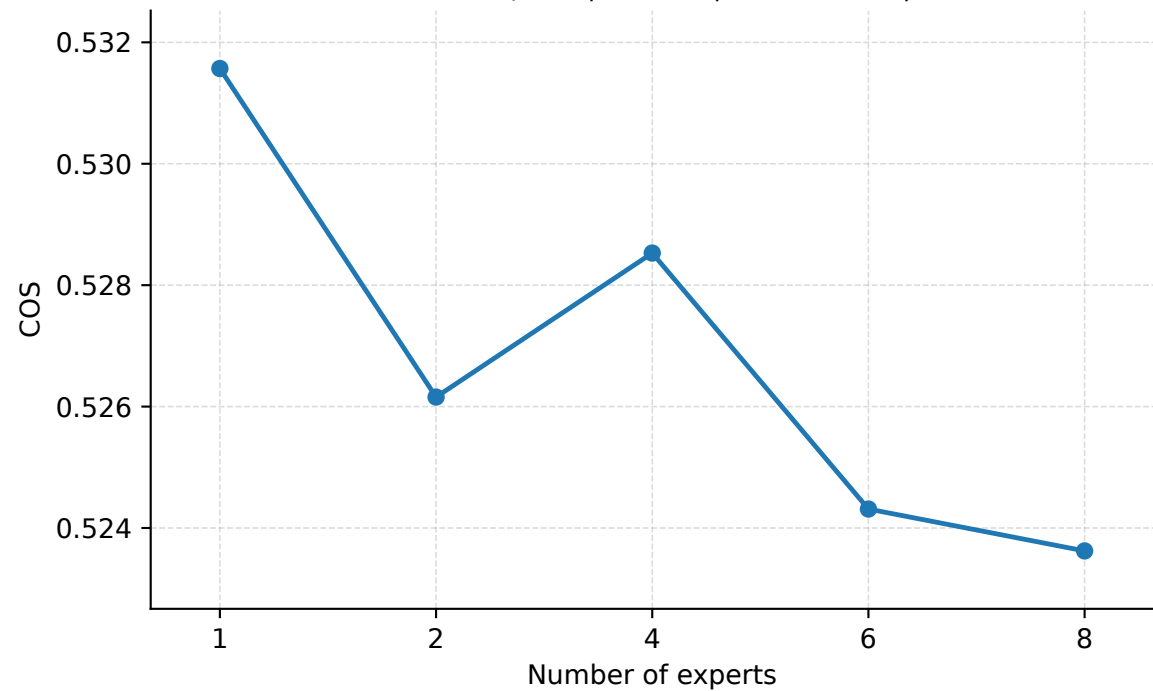
Number of Experts | Abilene | PredLen=10 | COS
