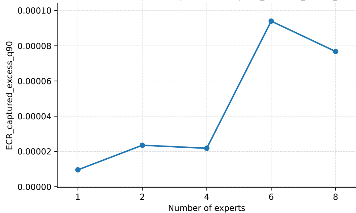
Number of Experts | Abilene | PredLen=10 | ECR_captured_excess_q90
