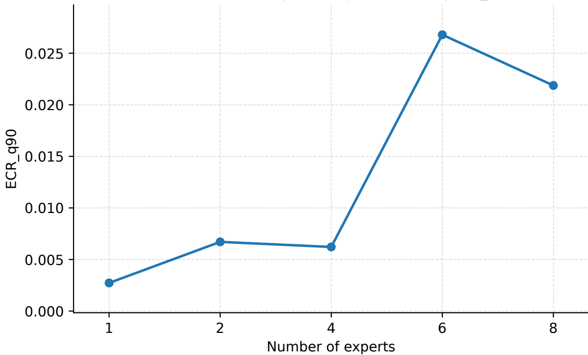
Number of Experts | Abilene | PredLen=10 | ECR_q90
