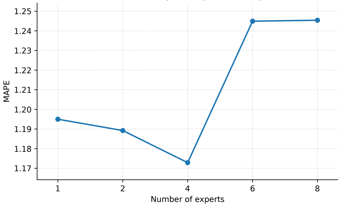
Number of Experts | Abilene | PredLen=10 | MAPE
