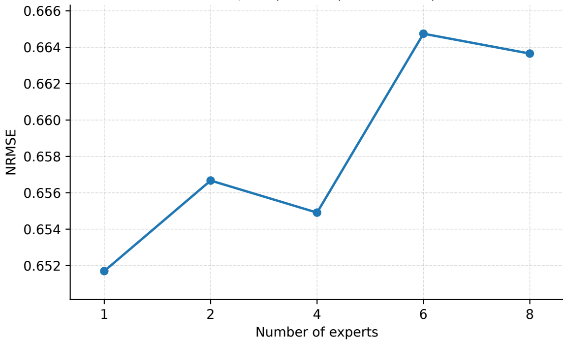
Number of Experts | Abilene | PredLen=10 | NRMSE
