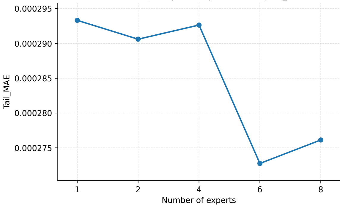
Number of Experts | Abilene | PredLen=10 | Tail_MAE
