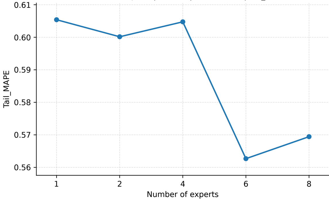
Number of Experts | Abilene | PredLen=10 | Tail_MAPE
