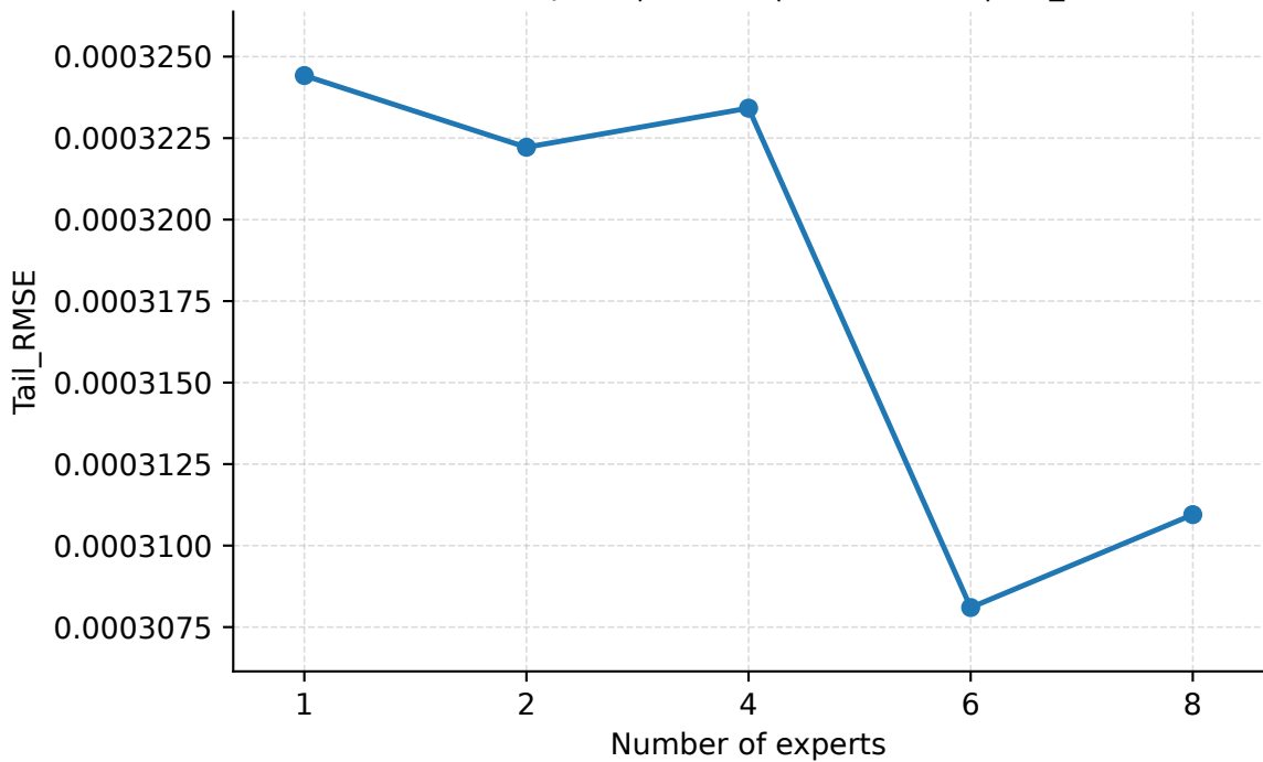
Number of Experts | Abilene | PredLen=10 | Tail_RMSE
