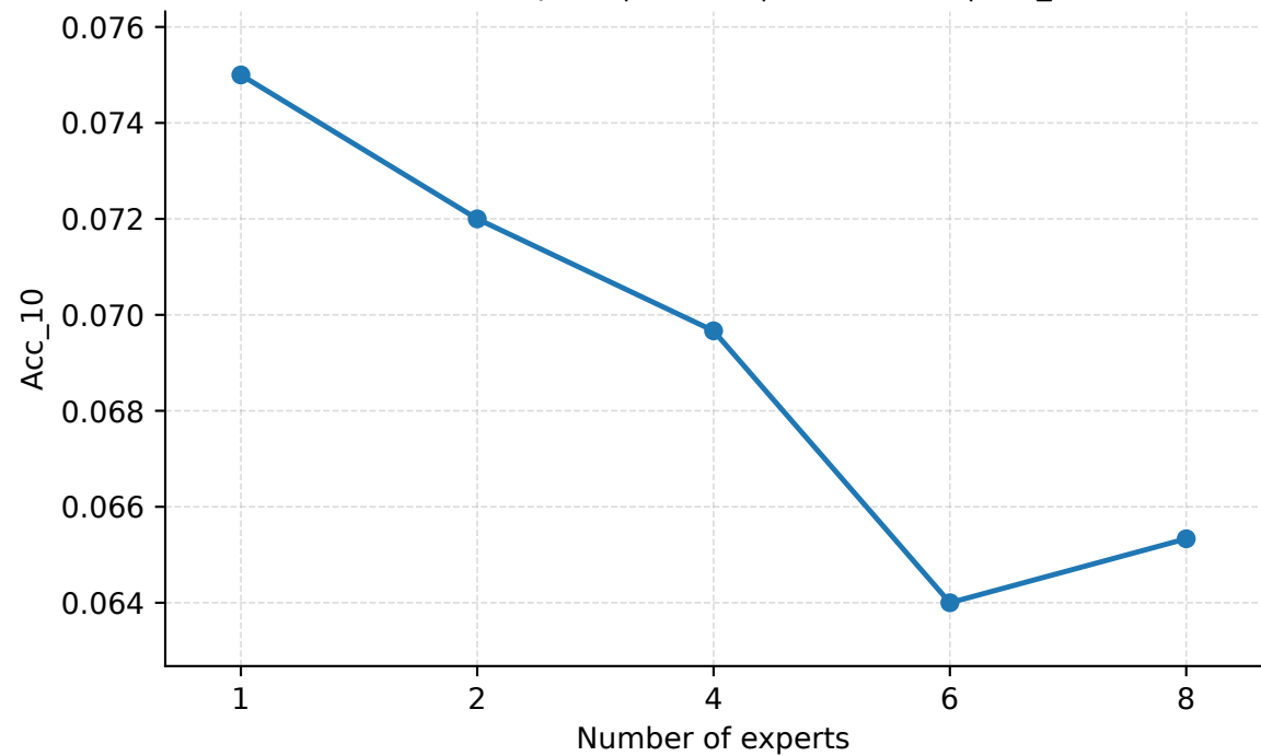
Number of Experts | Abilene | PredLen=15 | Acc_10
