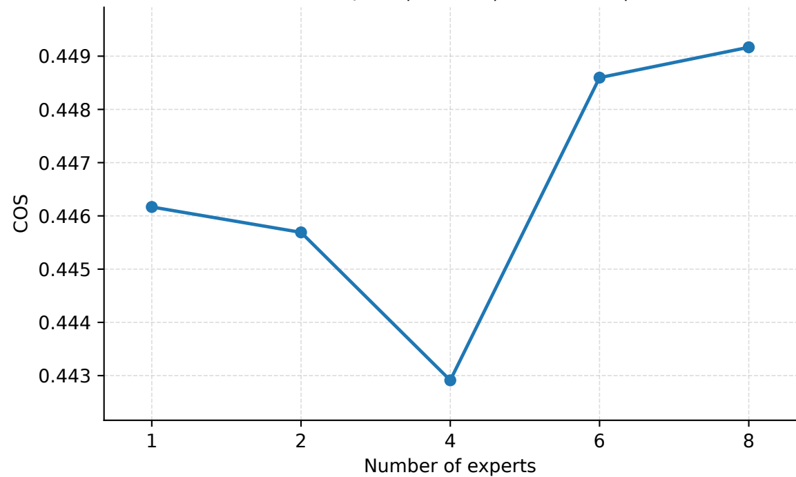
Number of Experts | Abilene | PredLen=15 | COS
