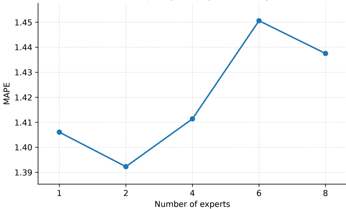
Number of Experts | Abilene | PredLen=15 | MAPE
