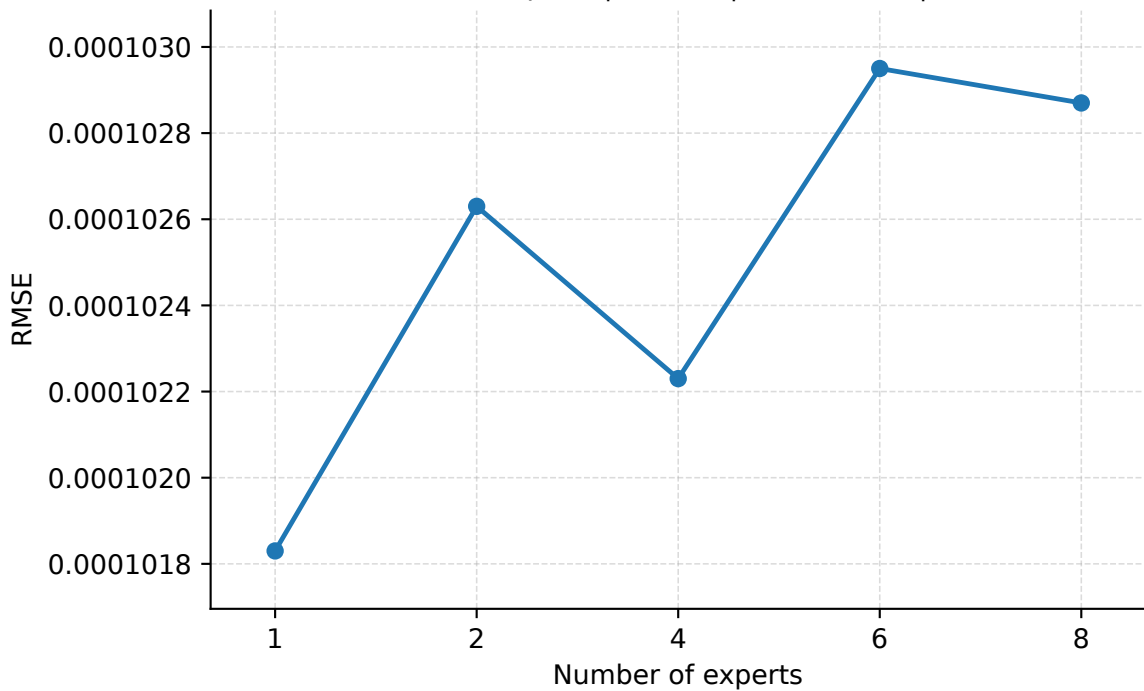
Number of Experts | Abilene | PredLen=15 | RMSE
