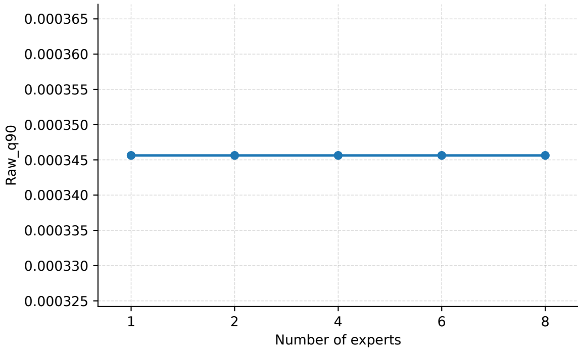
Number of Experts | Abilene | PredLen=15 | Raw_q90
