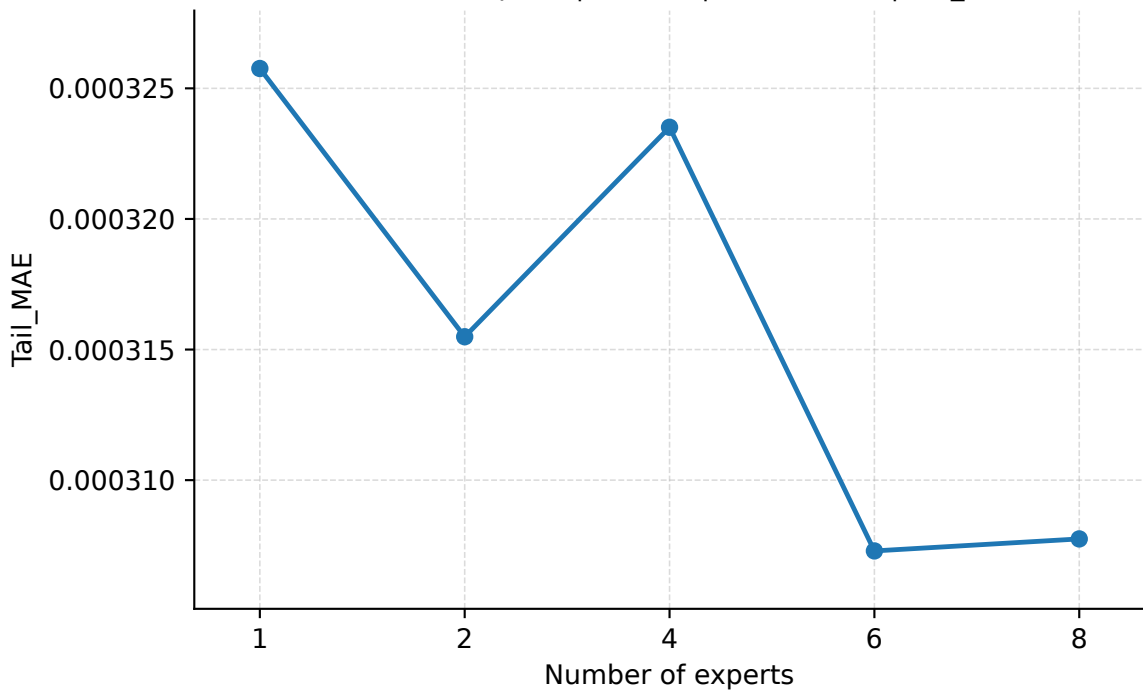
Number of Experts | Abilene | PredLen=15 | Tail_MAE
