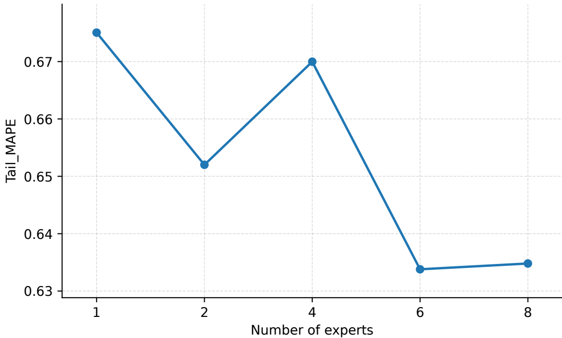
Number of Experts | Abilene | PredLen=15 | Tail_MAPE
