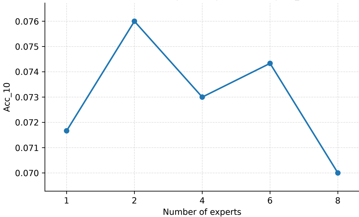
Number of Experts | Abilene | PredLen=20 | Acc_10
