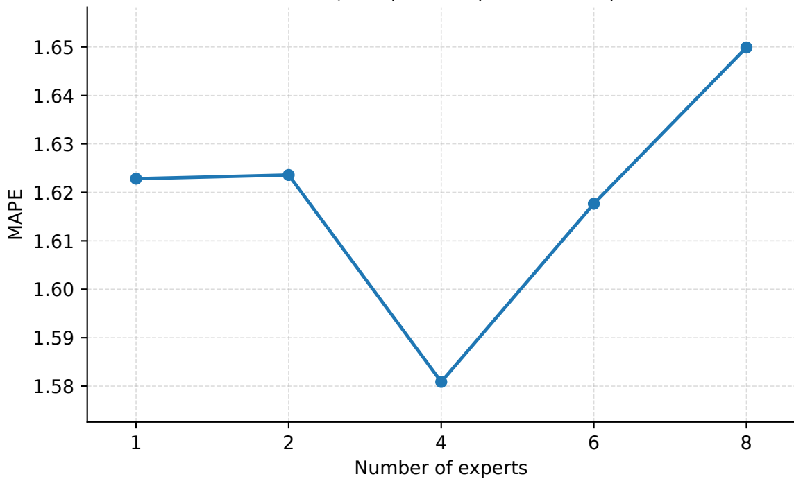
Number of Experts | Abilene | PredLen=20 | MAPE
