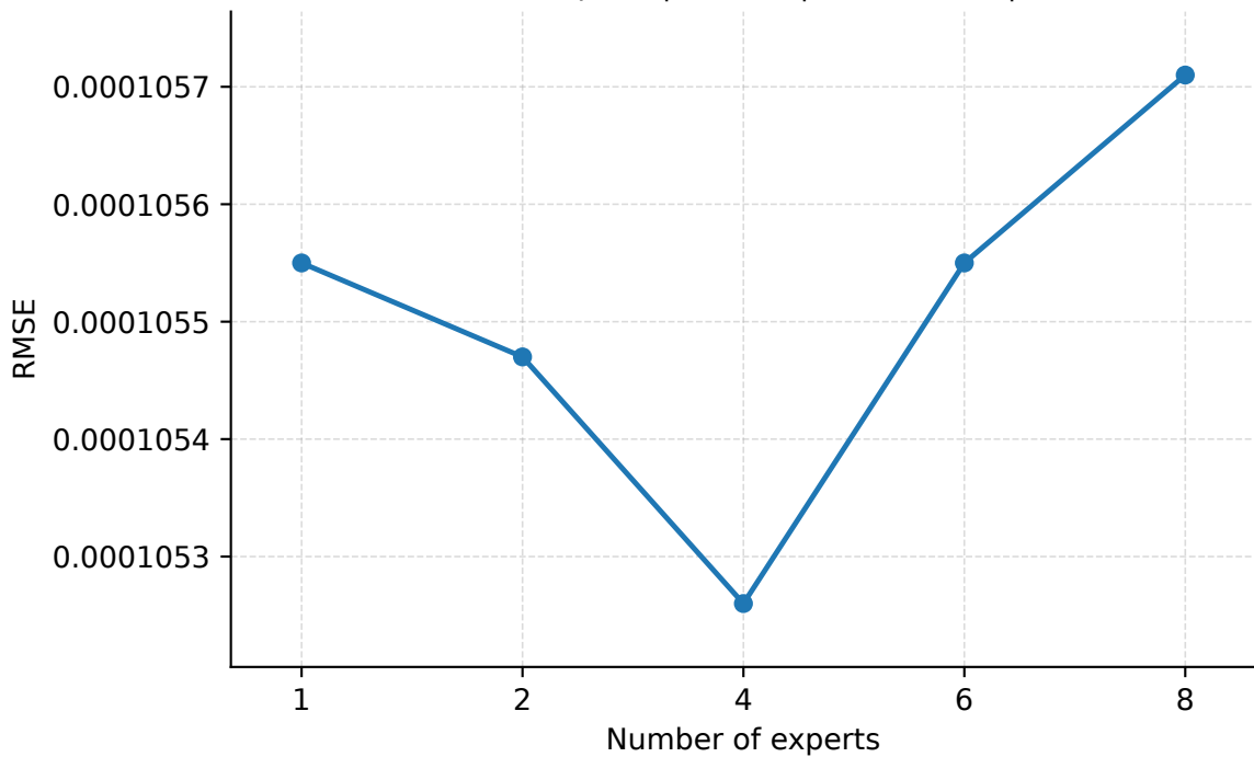
Number of Experts | Abilene | PredLen=20 | RMSE
