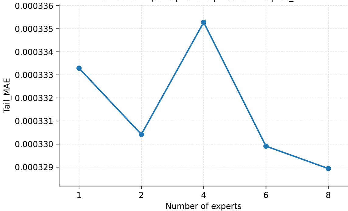
Number of Experts | Abilene | PredLen=20 | Tail_MAE
